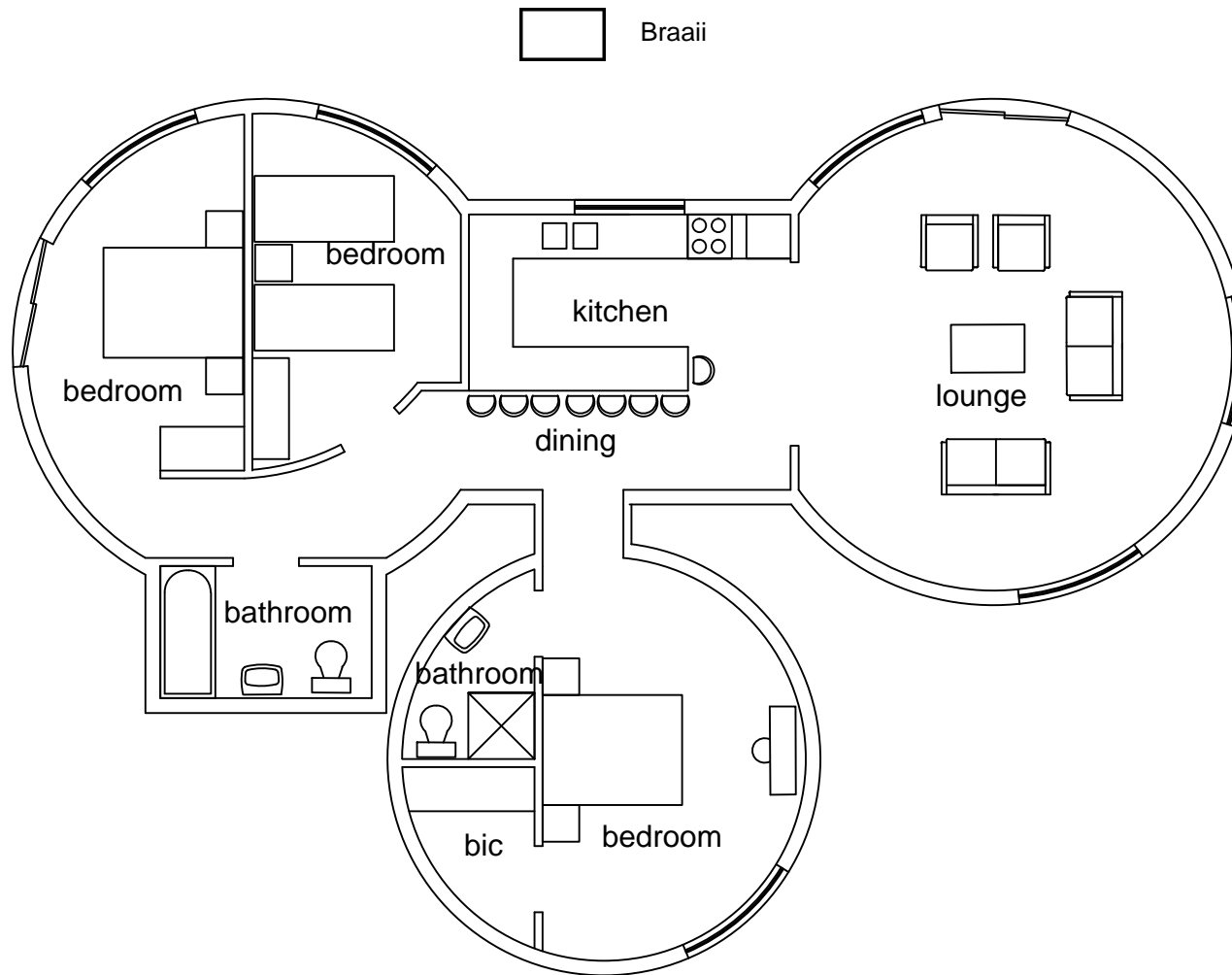
FLOOR PLAN 3 BEDROOM SUPERIOR CHALET CHALET 21 HOLE IN THE WALL
